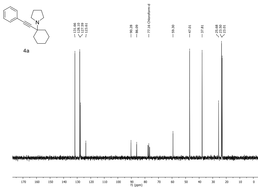
PICTURE 27: 13 C NMR for 1-(1-(phenylethynyl)cyclohexyl)pyrrolidine 4a
