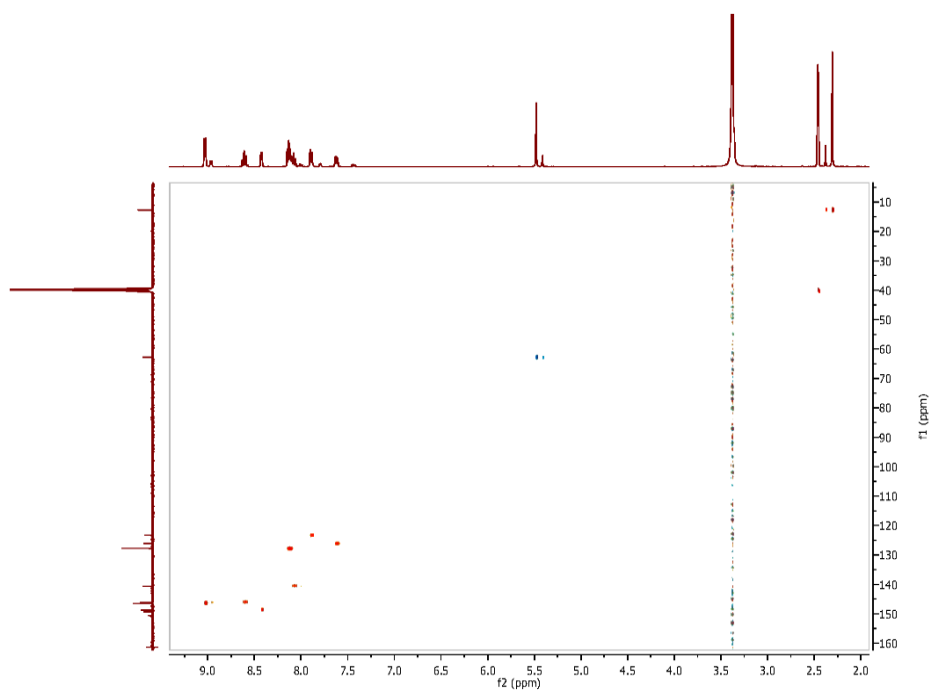
PICTURE 25: HSQC NMR Spectra for complex 6 [ \text{ZnL}^4(\text{N}_3)_2 ]
