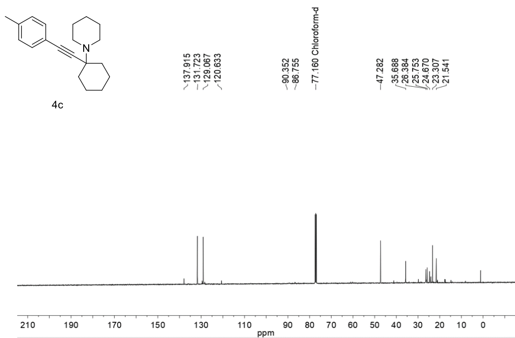
PICTURE 31: ^{13}\text{C} NMR for 1-(1-(p-tolylethynyl)cyclohexyl)piperidine 4c
