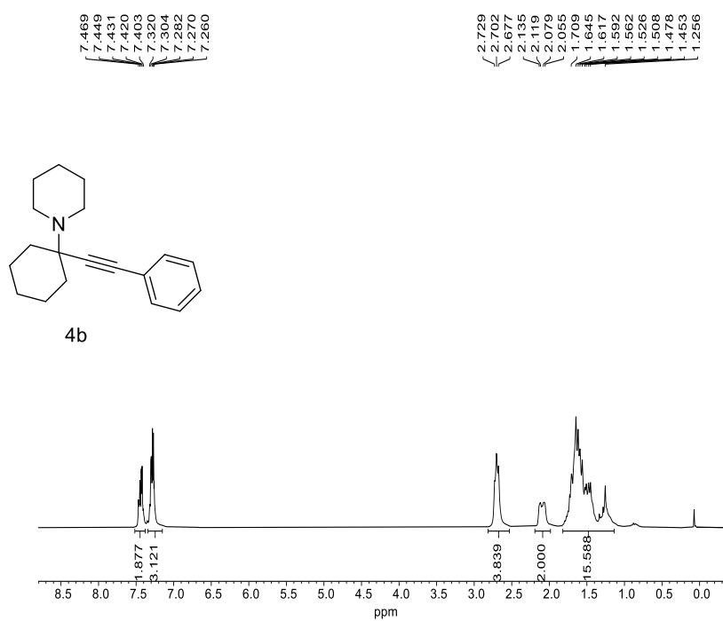
PICTURE 28: 1 H NMR for 1-(1-(phenylethynyl)cyclohexyl)piperidine 4b
