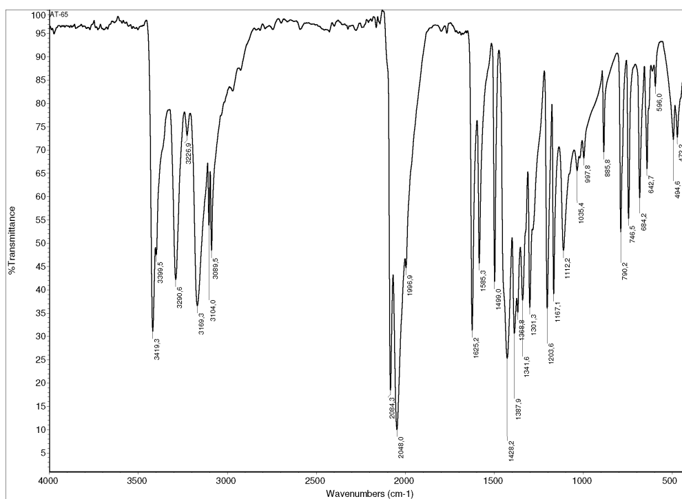
PICTURE 16: IR Spectra for complex 5 [\text{ZnL}^2(\text{N}_3)_2]
