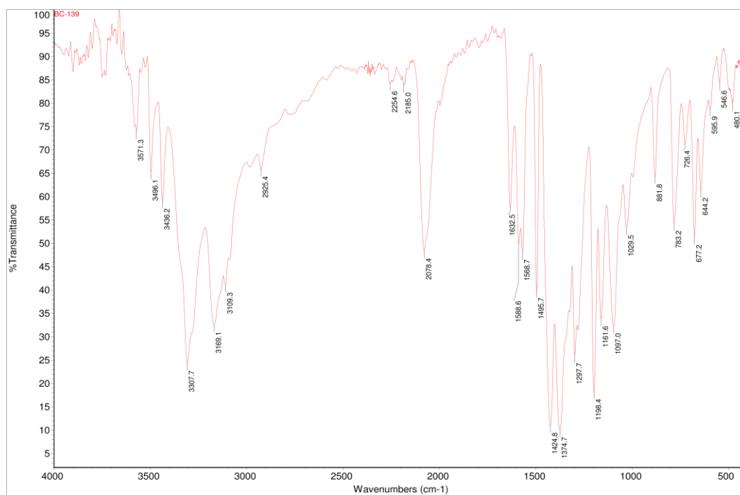
PICTURE 13: IR Spectra for complex 2 [\text{Zn}(\text{L}^2)_2]
