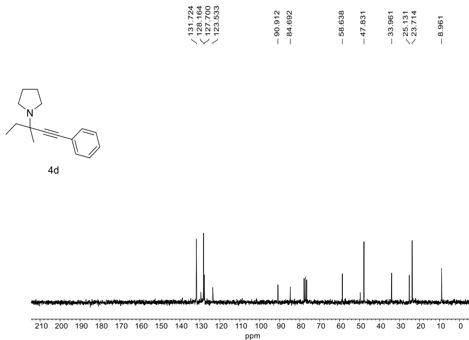
PICTURE 33: 13 C NMR for 1-(3-methyl-1-phenylpent-1-yn-3-yl)pyrrolidine 4d
