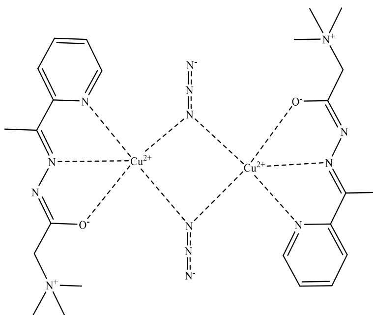
Figure 13: Representation of (11) [\text{Cu}_2\text{L}^3_2(\mu\text{-1,1-N}_3)_2]
