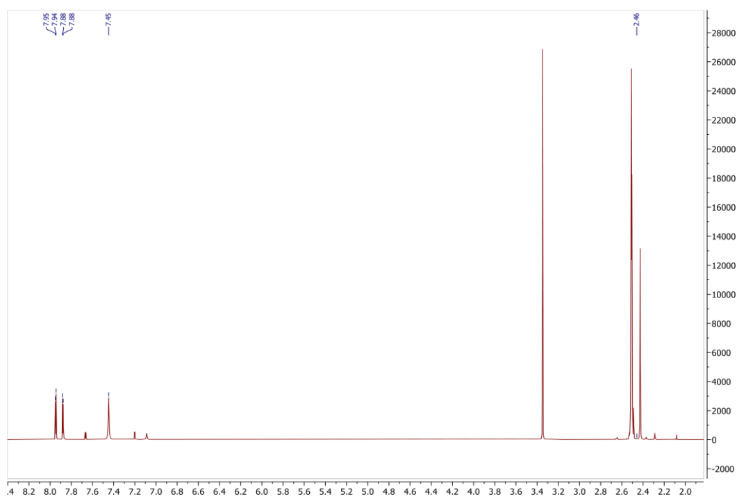
PICTURE 14: 1 H NMR Spectra for complex 2 [\text{Zn}(\text{L}^2)_2]
