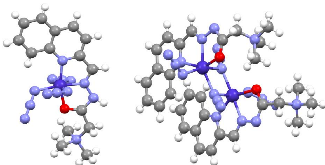
Figure 16: Representation of (14) [\text{CoHL}^5(\text{N}_3)_3] and (15) [\text{Co}_2\text{L}^5_2(\mu\text{-}1,1\text{-N}_3)_2(\text{N}_3)_2] respectively
