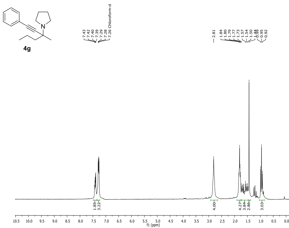
PICTURE 38: 1 H NMR for 1-(3-methyl-1-phenylhex-1-yn-3-yl)pyrrolidine 4g
