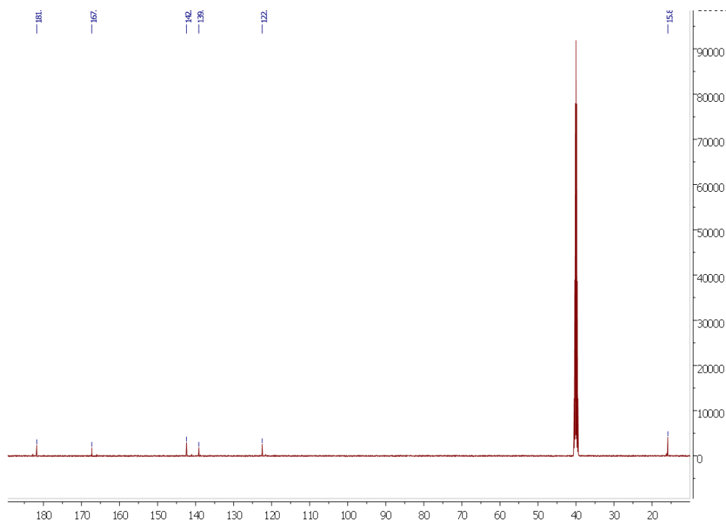
PICTURE 15: ^{13}\text{C} NMR Spectra for complex 2 [\text{Zn}(\text{L}^2)_2]
