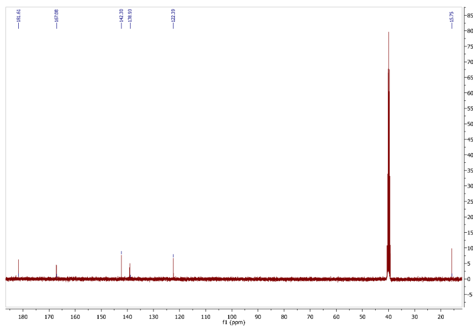
PICTURE 18: ^{13}\text{C} NMR Spectra for complex 5 [\text{ZnL}^2(\text{N}_3)_2]
