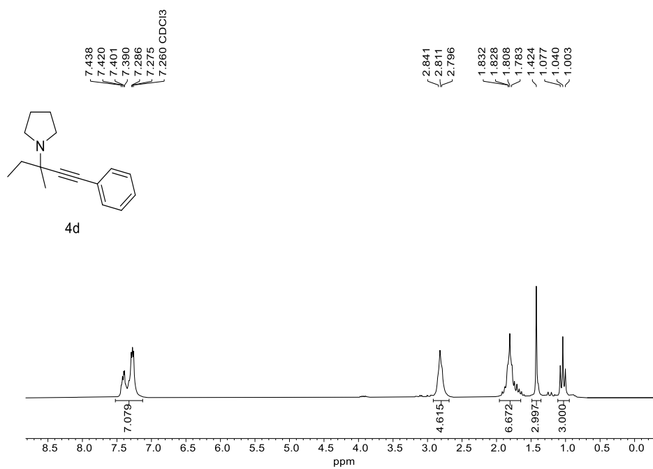
PICTURE 32: ^1\text{H} NMR for 1-(3-methyl-1-phenylpent-1-yn-3-yl)pyrrolidine 4d
