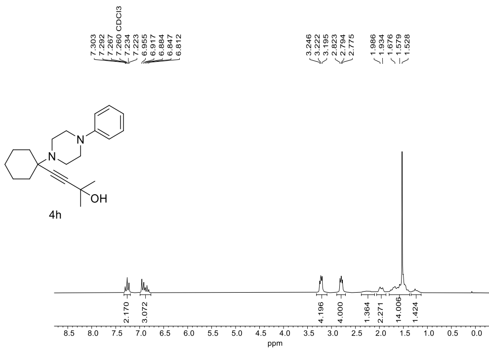
PICTURE 40: 1 H NMR for 2-methyl-4-(1-(4-phenylpiperazin-1-yl)cyclohexyl)but-3-yn-2-ol 4h
