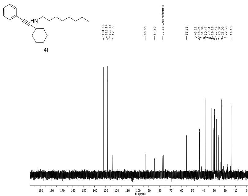
PICTURE 37: 13 C NMR for N -octyl-1-(phenylethynyl)cyclohexanamine 4f
