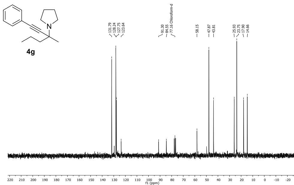
PICTURE 39: 13 C NMR for 1-(3-methyl-1-phenylhex-1-yn-3-yl)pyrrolidine 4g
