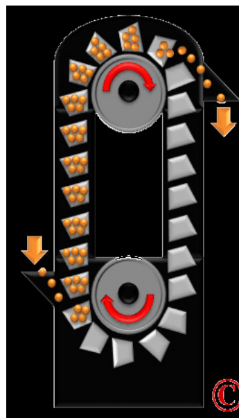
Figure 4.3: Bucket elevator
